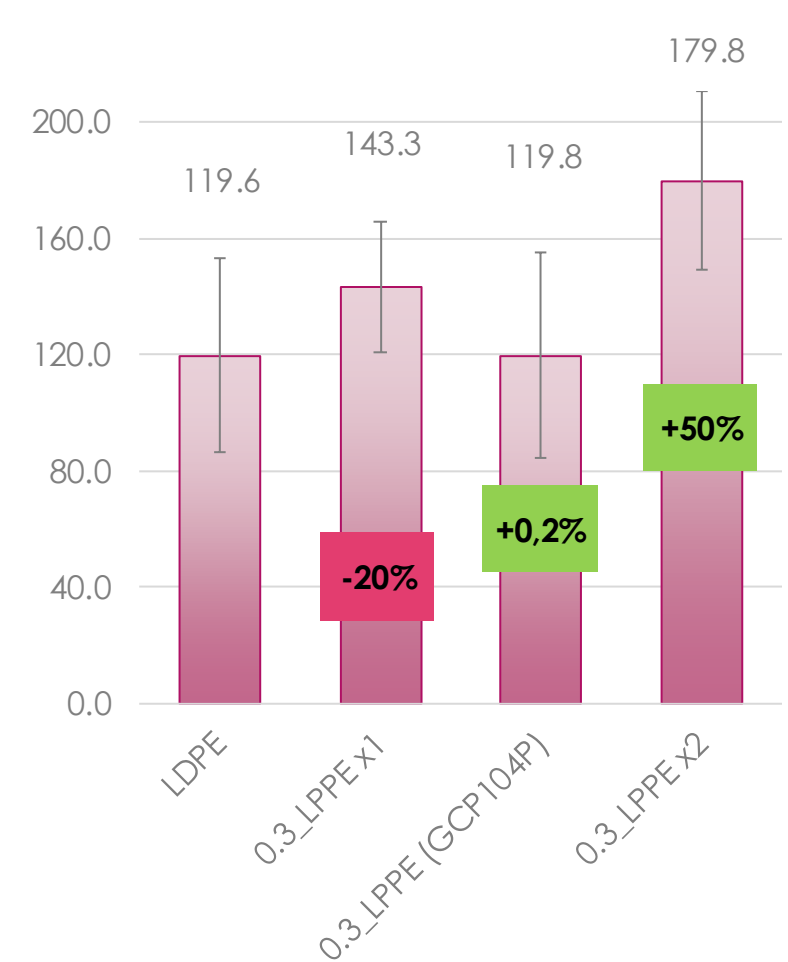
Total Elongation (%)
