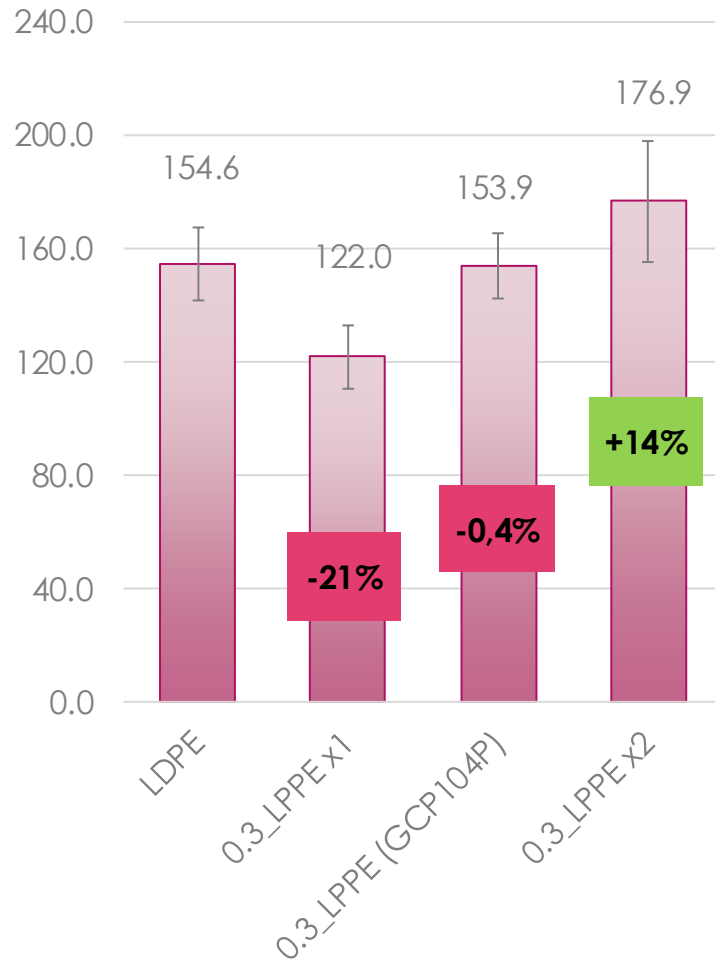
Young's Modulus (MPa)
